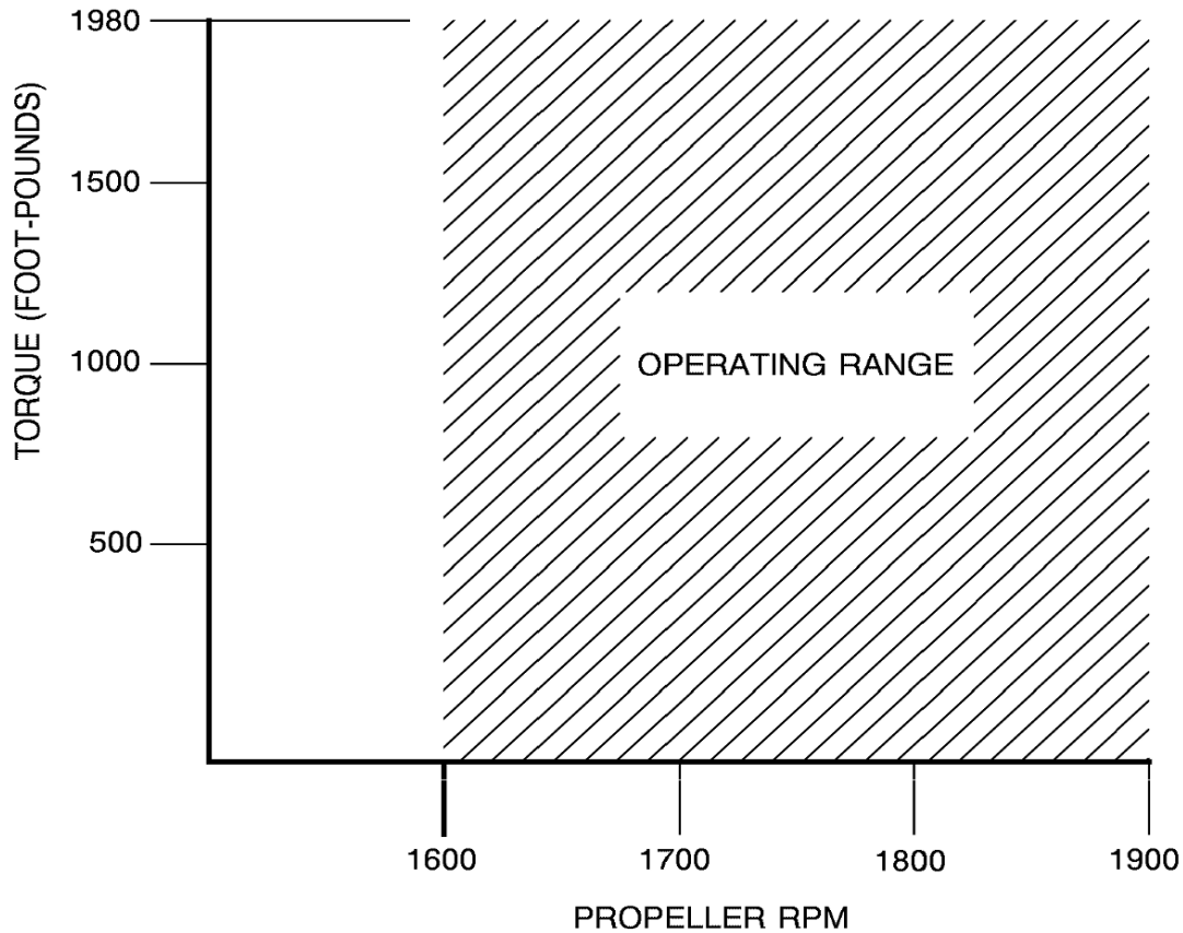
Figure 501 : Sheet 4 : Engine Operating Limits
