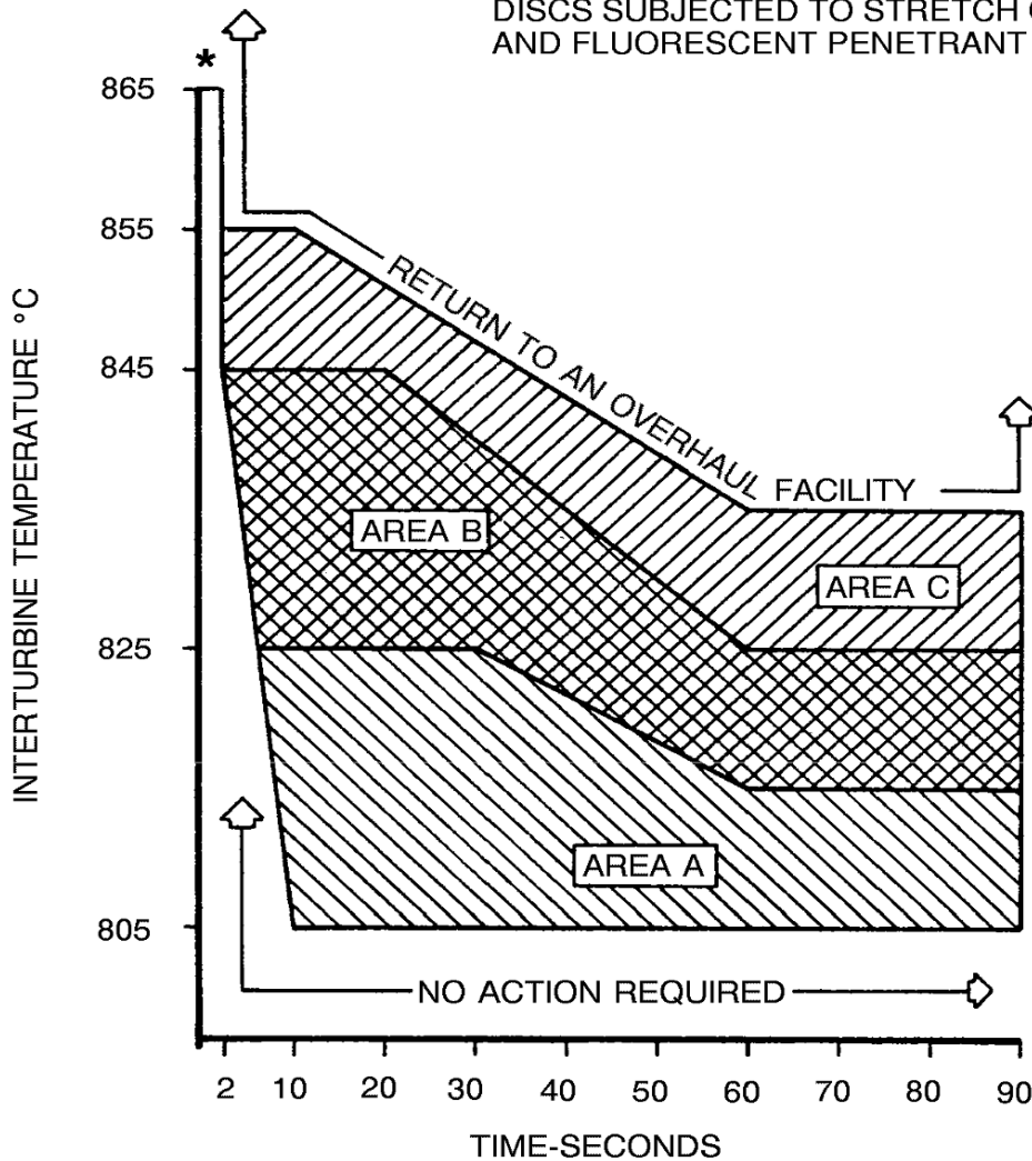
OVERTEMPERATURE LIMITS (ALL CONDITIONS EXCEPT STARTING) PT6A-114 AND PTA6A-114A
