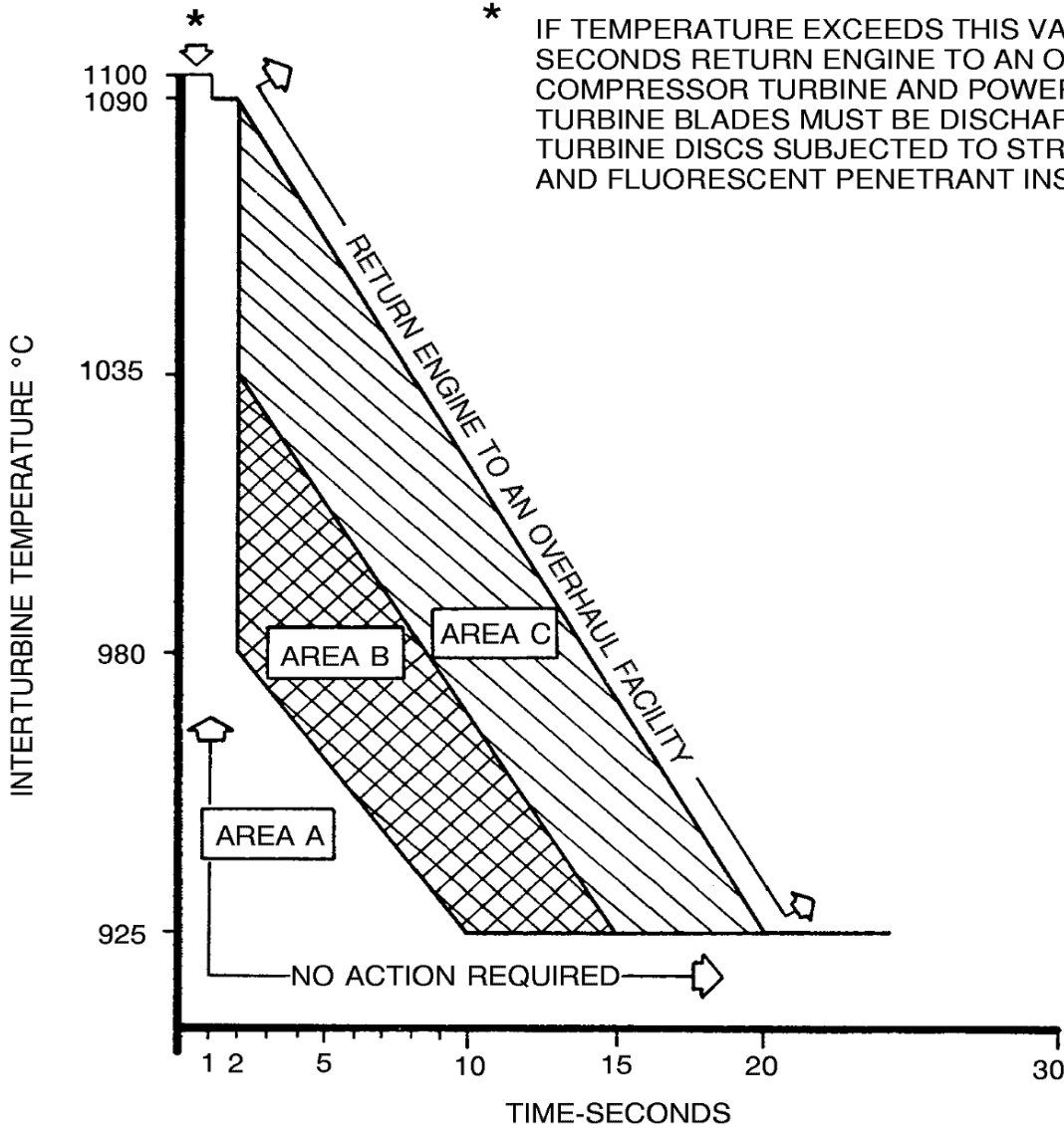
OVERTEMPERATURE LIMITS (STARTING CONDITIONS ONLY) PT6A-114 AND PT6A-114A
